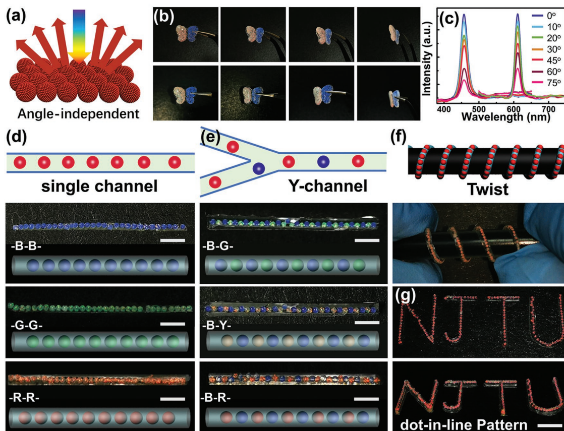
Figure 4. a) Cartoon illustration of angle-independence of the photonic gel. b) Photographs of a butterfly-shaped photonic gel at different viewing angles. c) Reflectance spectra of the red and blue part of the butterfly-shaped photonic gel at varying detection angles from 0° to 75°. d, e) Microfluidics-assisted assembly of linear photonic gel. Linear photonic gel with (d) one kind of colloidal crystal and (e) two kind of colloidal crystal were prepared by single and Y-type channel. Scale bar is 1 mm. f) 3D spiral photonic hydrogel. g) The optical images of structural color pattern prepared by injectable photonic precursor hydrogel solution. Scale bar is 2 mm.
