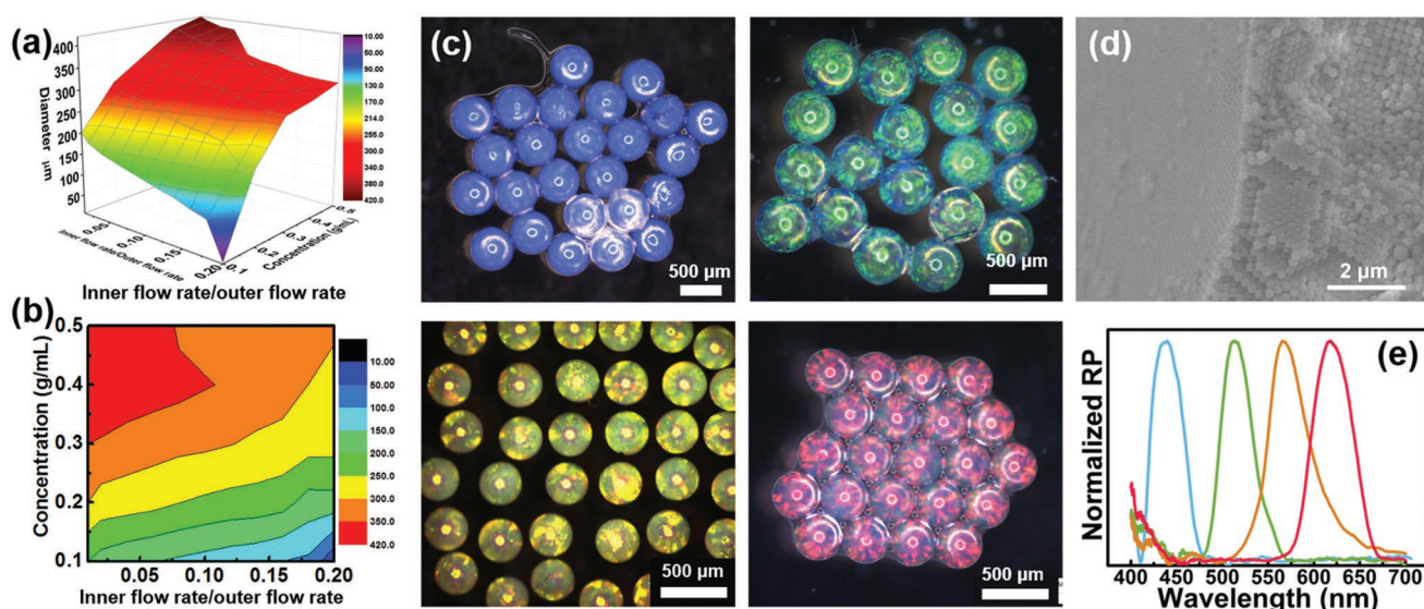
Figure 2. a,b) The relationship of diameter of photonic supraballs with inner and outer flow rate, and emulsion concentration. c) Optical micrographs of four photonic supraballs fabricated from PS@poly(HPA-co-VI) microspheres with different diameters. d) SEM image of the cross-section of a photonic supraballs. e) Reflection spectra of photonic supermicrospheres with different structural colors: blue (439 nm), green (514 nm), yellow (565 nm), and red (618 nm)
