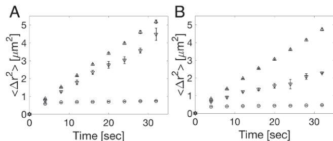
Fig. 5. MSD as a function of time for particles in the crystal ( \circ ), interface ( \nabla ), and liquid ( \Delta ). (A) BCC. (B) FCC.
