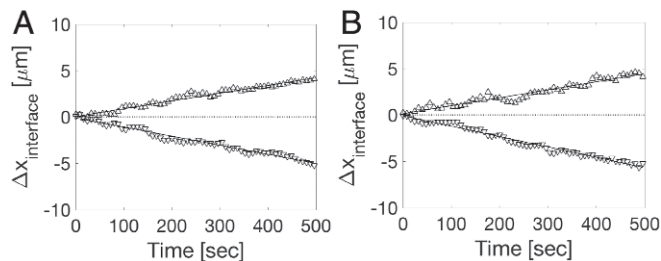
Fig. 4. Change in interface position during crystallization and melting. \Delta , crystal growth when the voltage is stepped from 0 to 80 V; \nabla , crystal melting when the voltage is stepped from 80 to 0 V. (A) BCC–liquid interface ( v_{\text{growth}} = 0.0087 \pm 0.0006 \mu\text{m/s} , v_{\text{melting}} = -0.0118 \pm 0.0013 \mu\text{m/s} ). (B) FCC–liquid interface ( v_{\text{growth}} = 0.0084 \pm 0.0004 \mu\text{m/s} , v_{\text{melting}} = -0.0099 \pm 0.0005 \mu\text{m/s} ).
