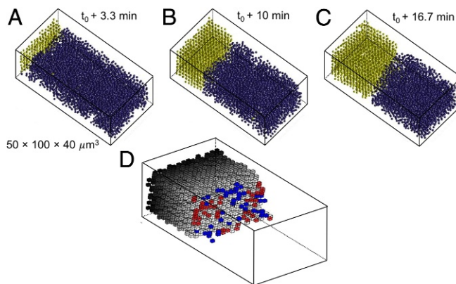
Fig. 2. Growth of a BCC crystal from the liquid. (A–C) Reconstructed images of the crystallization process, where yellow particles are crystalline and blue particles are liquid. (D) Identification over one imaging interval of 4 s of attachment (red) and detachment (blue) sites at the crystal boundary with the liquid. The interface particles have been removed for clarity.
