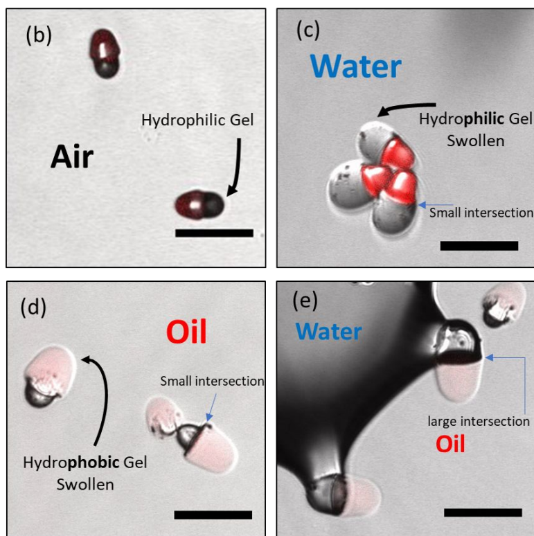
50 51 52 53 54 55 56 57 58 59 60 Figure 3. Swelling characteristics of the amphiphilic Janus microgels. (a) amount of absorbed water or toluene for the hydrophilic and hydrophobic sides respectively; swelling either individually in the pure solvents or simultaneously at the water/toluene interface. (b) Janus microgel sitting in air. (c) Janus microgel sitting in water with the hydrophilic side swollen. (d) Janus microgel sitting in toluene with the hydrophobic gel swollen. (e) Janus microgel sitting at the interface of a water drop in toluene with
