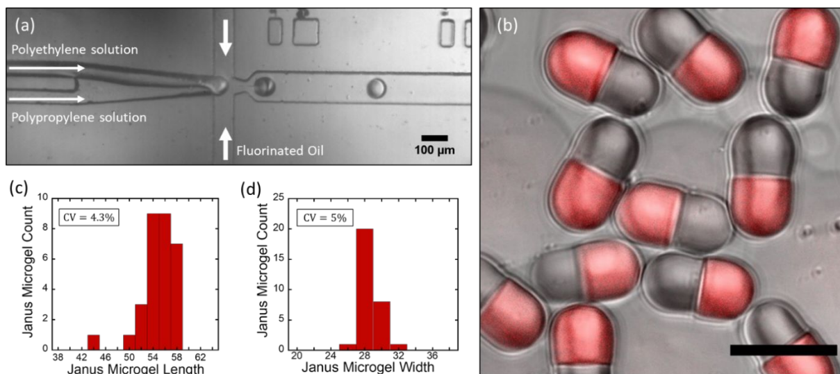
Figure 1. Fabrication of Janus Microgels (JMs). (a) Janus droplet formation of polymer precursor solutions via shear by fluorinated oil in microfluidic flow-focusing device. (b) synthesized amphiphilic Janus microgels showing the distinctive hydrophilic (gray) and hydrophobic (red) sides washed and submerged in acetone. Scale bar is 50 μm. (c) histogram of final length (hydrophobic edge to hydrophilic) of Janus microgels (average 56 μm) with coefficient of variation (CV) as standard deviation/average length. (d) histogram of final width (particle intersection) of Janus microgels (average 28.5 μm) with coefficient of variation (CV) as standard deviation/average length.
