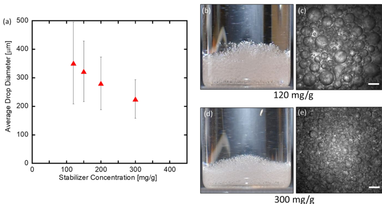
Figure 4. Changing emulsion droplet size with amount of JM stabilizers. (a) drop diameter as a function of particle concentration for water in toluene emulsions. (b) water in toluene emulsions sedimented on the bottom of the vial due to density differences using 120mg JM to 1g of water. (c) optical micrographs of the emulsion droplets at 120 mg/g concentration. (d) water in toluene emulsions on bottom of vial with 300mg JM to 1g of water. (e) optical micrographs of the emulsion droplets at 300 mg/g concentration. Scale bars are 500 \mu\text{m} .
