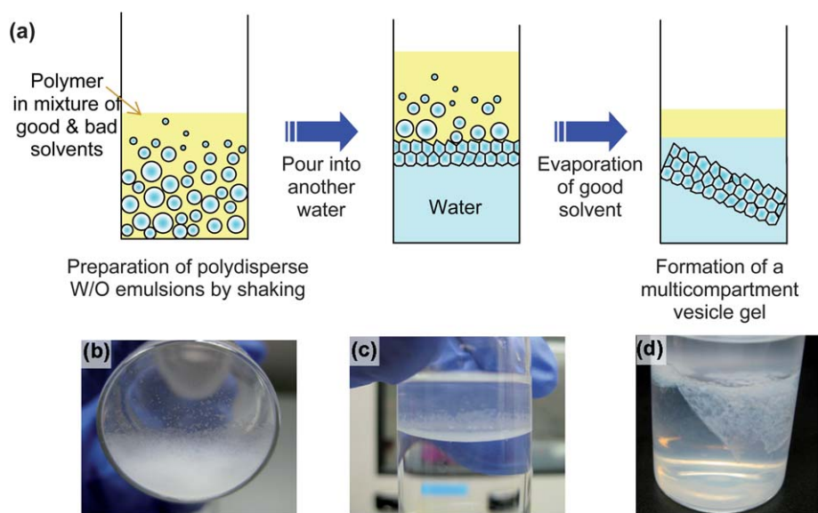
Fig. 1 (a) Schematic of the fabrication of multicompartiment vesicle gel; (b–d) photographs of (b) a water-in-oil (W/O) emulsion with water droplets dispersed in a mixture of chloroform and hexane (36 : 64 v/v) with 10 mg mL -1 PEG(5000)- b -PLA(5000) dissolved in it, (c) the same W/O emulsion floating on a layer of water, and (d) the resultant polymersome gel.
