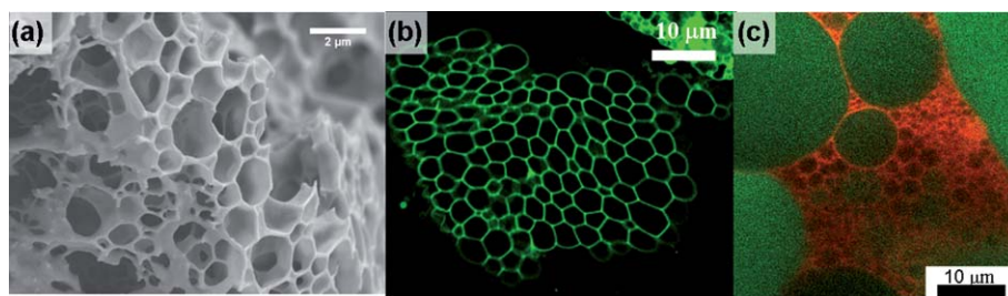
Fig. 2 (a) Scanning electron microscope (SEM) image of a dried vesicle gel; (b–c) confocal laser scanning images of (b) multicompartment vesicle gels with NBD-cholesterol in the membrane walls separating the compartments, and (c) multicompartment vesicle gels with FITC-Dextran inside the compartments and a trace amount of pyromethene 605 in the membrane walls.
