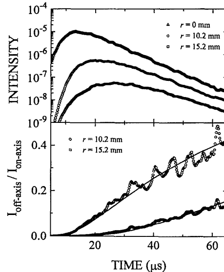
FIG. 6. Comparison of the transmitted intensity I(t) measured with the detector displaced a distance r away from the axis of the source to that measured with the detector placed directly on axis. The solid curves in the lower panel show the expected exponential reduction in the ratio of off-axis to on-axis intensity and give a measure of D that is independent of absorption and boundary effects.
