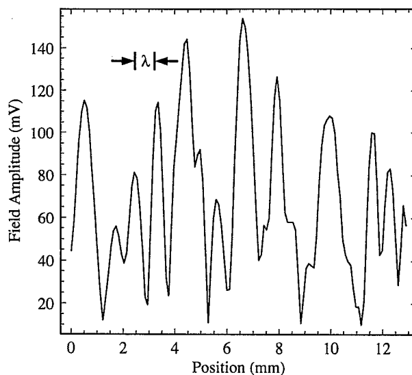
FIG. 1. Cross section of the acoustic speckle pattern of multiply scattered sound transmitted through a 20-mm-thick sample containing 0.5-mm-radius glass beads immersed in water. The speckle pattern was detected in the near field. The coherence area is approximately \lambda^2 , where \lambda=0.6 mm is the ultrasonic wavelength in water.
