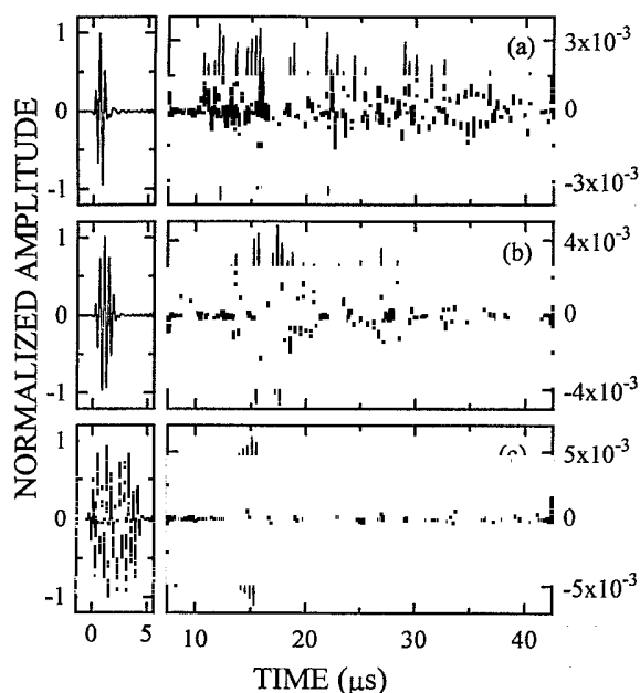
FIG. 2. Time evolution of the transmitted ultrasonic fields in a single speckle (right) for three different incident pulse widths (left), showing the temporal fluctuations of the multiply scattered fields.
