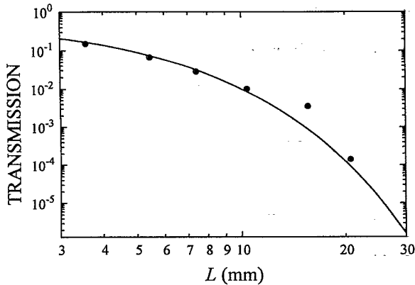
FIG. 8. Dependence of the absolute transmission on sample thickness L . The incident ultrasonic beam was generated using the plane-wave geometry with a sufficiently long pulse that continuous-wave conditions were obtained to an excellent approximation. The fit to Eqs. (6) and (7), shown by the solid curve, gives l^* = 0.8 \pm 0.05 mm.
