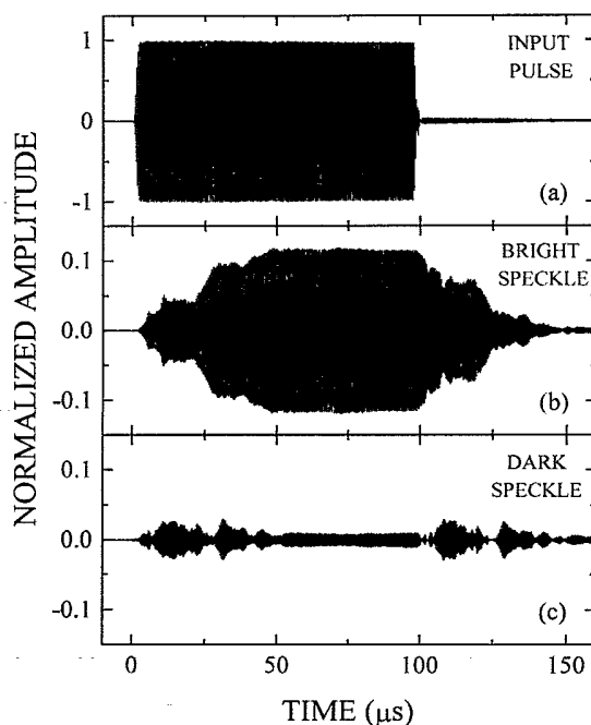
FIG. 3. Transmitted ultrasonic field in a single speckle for an incident pulse width of 100 \mu\text{s} . The incident pulse is shown in (a) and the transmitted fields in typical bright and dark speckles are shown in (b) and (c). Note the region from about 60 to 100 \mu\text{s} , where the amplitude is essentially flat, corresponding to the quasi-continuous-wave case in which the entire distribution of allowed path lengths are filled.
