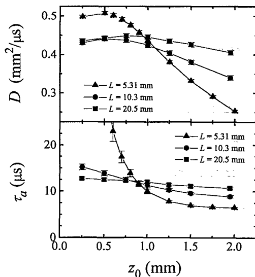
FIG. 5. Dependence of the fitted parameters D and \tau_a on the penetration depth z_0 for the data shown in Fig. 4. The consistency of the fitted parameters for z_0 between 0.7 and 1 mm gives an estimate for l^* of 0.85 \pm 0.2 mm.
