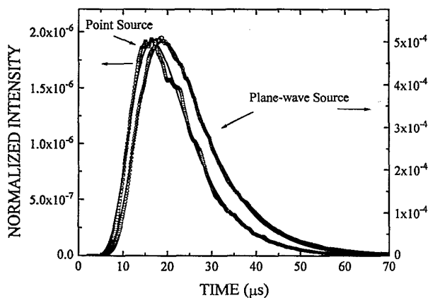
FIG. 7. Comparison of the time profile of the transmitted intensity for a point source and a plane-wave source. The smooth solid curves are fits to the corresponding expressions given by diffusion theory and provide another check of the applicability of the diffusion approximation.
