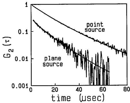
FIG. 1. Intensity autocorrelation functions vs time for transmission through 2-mm-thick cells with 0.497- \mu\text{m} -diam polystyrene spheres and \phi = 0.01 . Smooth lines are fits to the data by Eqs. (2) and (3) with l^* = 143 \mu\text{m} for the point source and l^* = 144 \mu\text{m} for the plane source.
