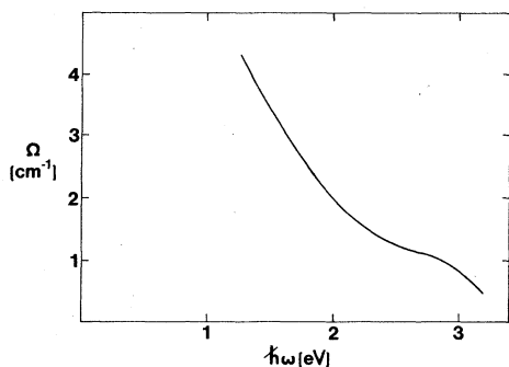
FIG. 8. Calculated \Omega as a function of \omega_{\text{ex}} for Brillouin scattering from a composite medium consisting of silver spheres in water. The concentration of spheres q is assumed to be inhomogeneous. The theory used is not valid for the regimes that produce the higher \Omega ( \lesssim 2.1 eV), and the results shown only illustrate the extrapolation (see Table I).
