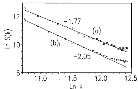
FIG. 3. Logarithmic plot of S(k) for clusters aggregated with (curve a ) diffusion-limited kinetics and (curve b ) reaction-limited kinetics. The fractal dimensions are (curve a ) 1.77 and (curve b ) 2.05. The units of k are \mu\text{m}^{-1} .
